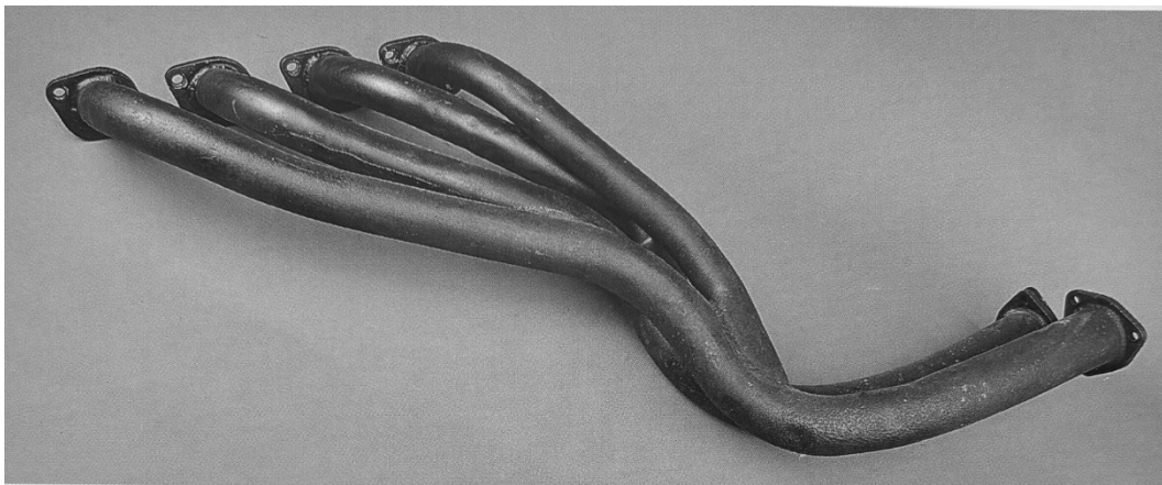
Exhaust manifold | Krümmer 105.16.01.071.00 / 105.16.01.072.00
